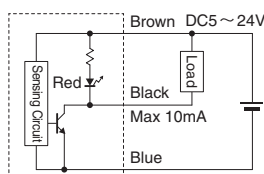
Circuit system CNC-2
