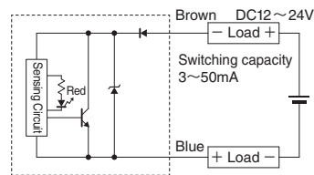
Circuit system CNC-8
