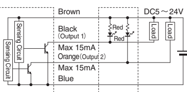
Circuit system CNC-20
