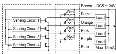
Circuit system CNC-13
