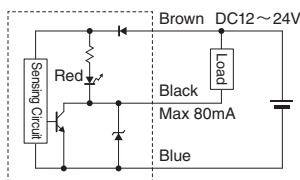
Circuit system CNC-16
