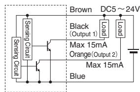
Circuit system CNC-6
