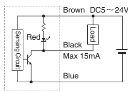
Circuit system CNC-7
