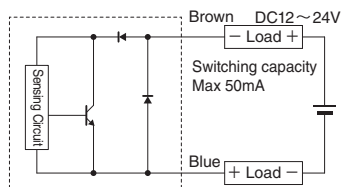
Circuit system CNC-19
