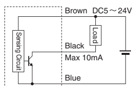
Circuit system CNC-1
